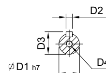
B-B SECTION (Output Shaft)
